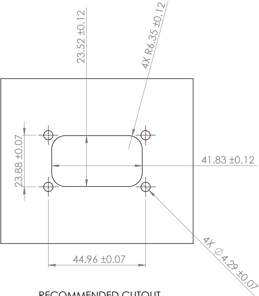
RECOMMENDED CUTOUT FRONT AND REAR MOUNT
