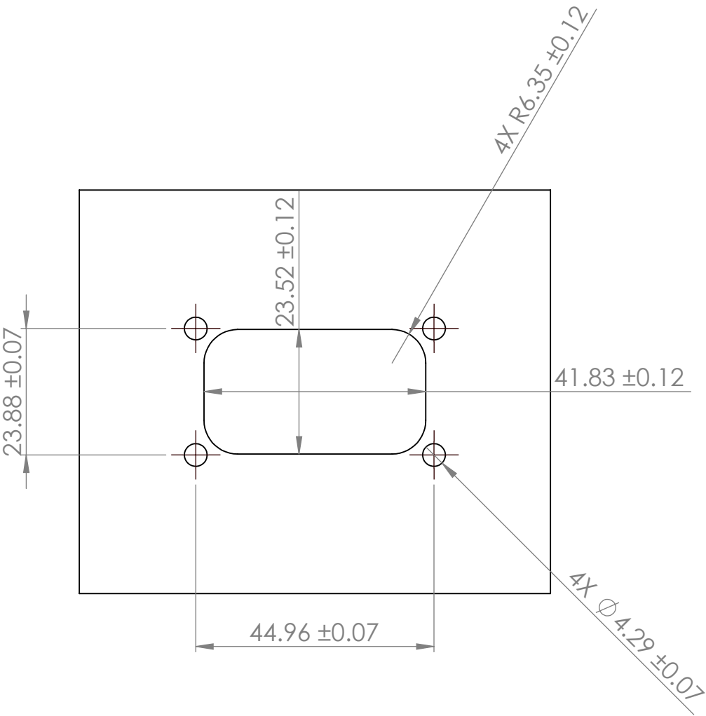
RECOMMEDED CUTOUT FRONT AND REAR MOUNT
