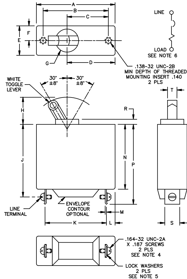
FIGURE 1. Dimensions and configurations (configuration 1).
