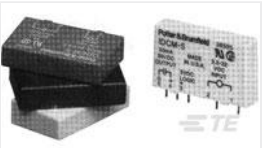
TE Part #1-1393028-2 IACM-5E = SLIM PCB MONT,5VDC Logic-AC ip
