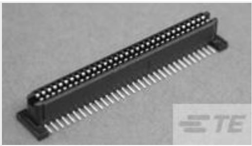
TE Part # 1-5120521-1 1FHR,64,50A/S,S,N,S08,09,10
