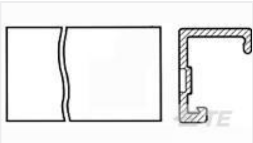
TE Part #4-640426-5 15P MTA156 CONN ASSY 18AWG ORA
