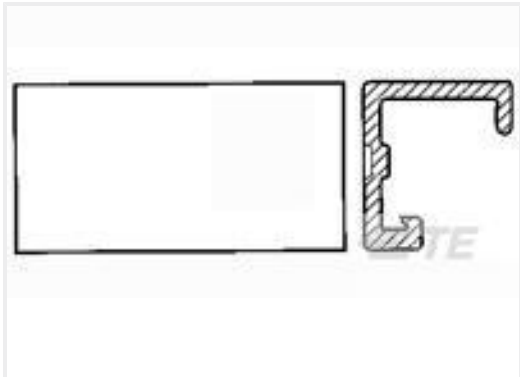
TE Part #640550-5 05P MTA100 COVER
