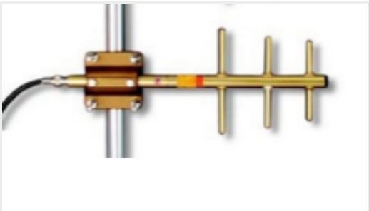
TE Part #Y8963 YAGI,FWG,3,896-970MHz, 6dBi
