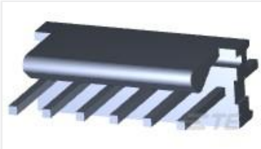
TE Part #3-641215-6 06P MTA100 HDR ASSY FL/ST 30AU
