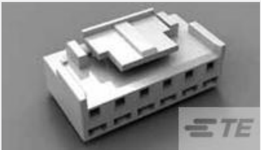
TE Part #3-770476-1 SL156 RECPT, SNNI/PHBZ
