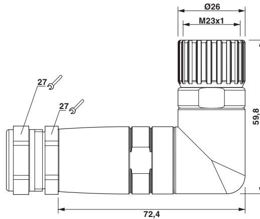
Dimensional drawing
