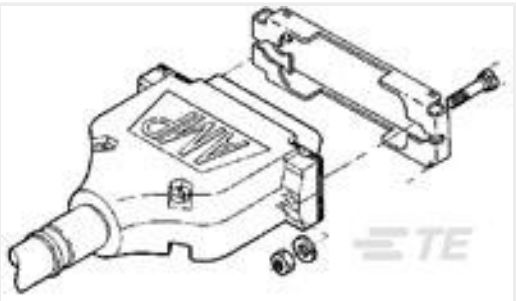
TE Part #5745584-1 UNIV SLIDLTCH KIT SZ 3
