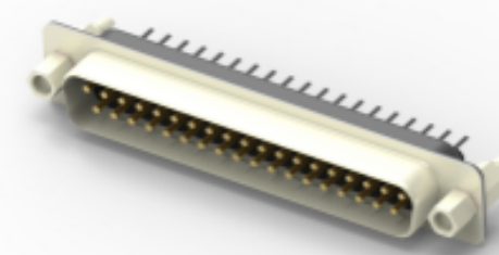
TE Part #2301836-1 AMPL PLUG HD20, VERT, 37P, B/L, 4-40 S/LO
