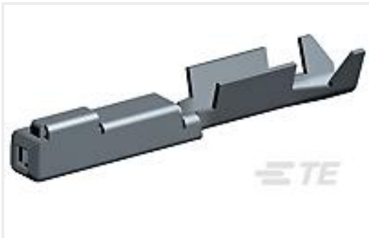
TE Part #1612290-1 0.64 RCPT SEALED TIN STRIP
