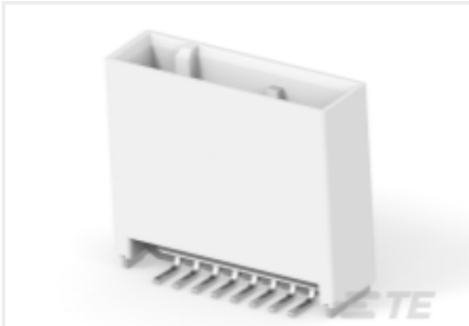
TE Part #2311396-2 8POS,TAB0.5X0.4,HDR ASSY,180DEG,COD B
