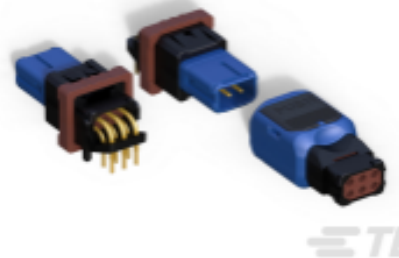
TE Part #YD369-B99-NS400000 369 9 WAY PANEL MNT REC, 90 PCB GOLD,SKT
