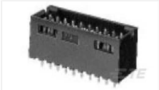
TE Part #7-103168-3 50 MODII HDR DRST SHRD .100CL
