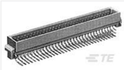
TE Part #5650478-5 ASSY,PIN,EUROCARD,TYPE C/2,LEA
