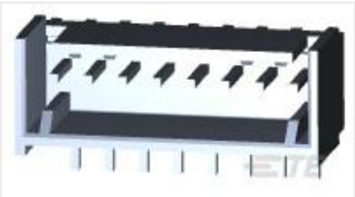
TE Part #2-644803-8 08P MTA100 SHRD HDR ASSY RA FL
