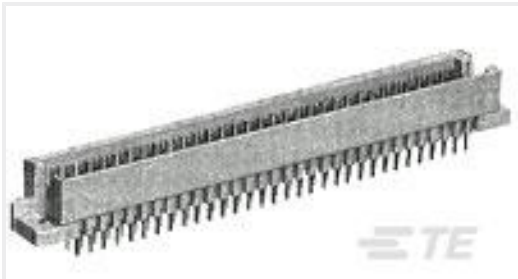
TE Part #5650470-5 ASSY,PIN,EUROCARD,TYPE R,LEAD-
