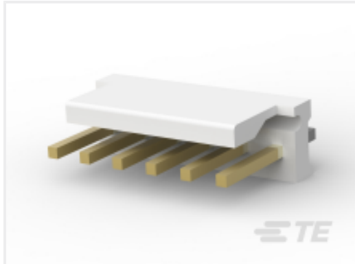
TE Part # 3-641208-6 06P MTA156 HDR ASSY FL ST LF
