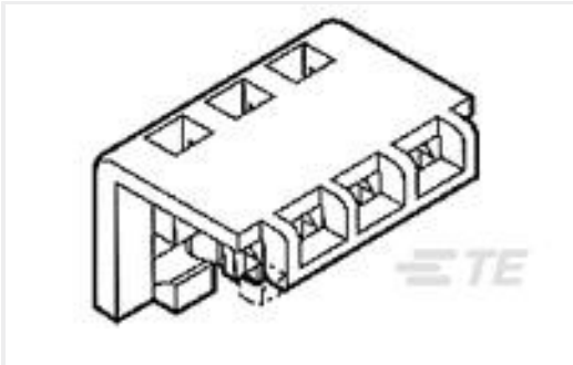
TE Part #1-643067-5 15P MTA156 MOLDED COVER
