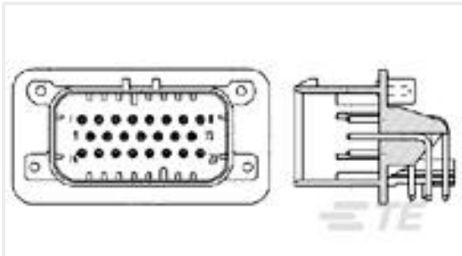
TE Part #776267-1 14POS,PIN DIA 1.3,HDR ASSY,90DEG, COD 1
