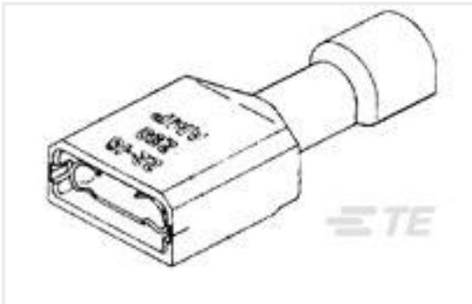
TE Part #3-520402-2 ULTRA-FAST 187 ASY REC 16-14 AWG TPBR
