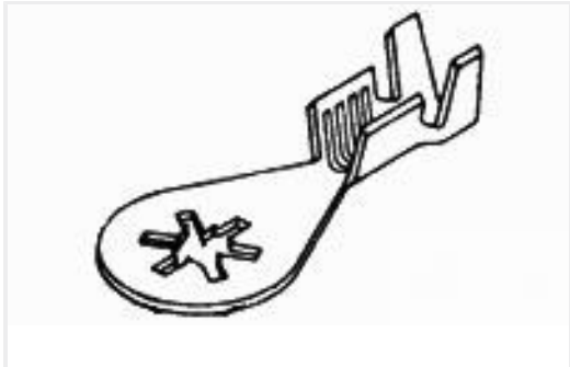
TE Part #61794-1 RING 18-14 AWG TPST
