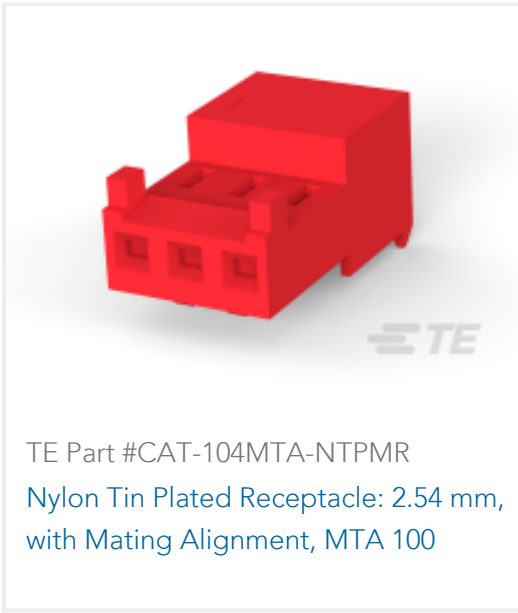
TE Part #640455-5 05P MTA100 HDR ASSY SQ R/A POL
