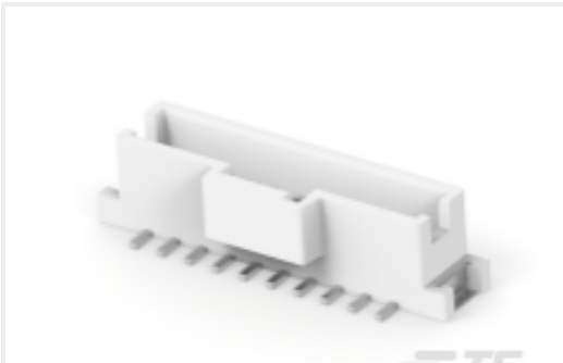
TE Part #2-2232829-0 SGI2.0 HEADER ASSEMBLY SMT 10P, KEY A,NTL
