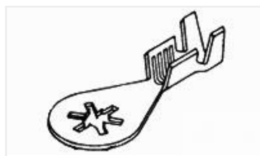
TE Part #62613-3 RING .190 12-10 AWG 024 TPCU
