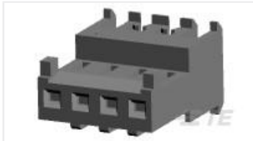
TE Part #3-644564-4 04P MTA100 CONN ASSY F/T 26AWG
