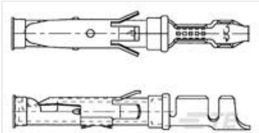
TE Part #163088-1 062 SOC.ASS. TYP3+
