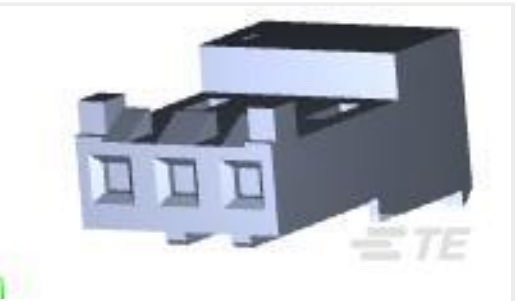
TE Part #3-643819-3 03P MTA156 CONN ASSY 22AWG RED
