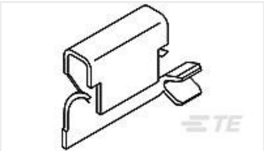
TE Part #63733-3 GROUND CLIP 18-22AWG TPPBR
