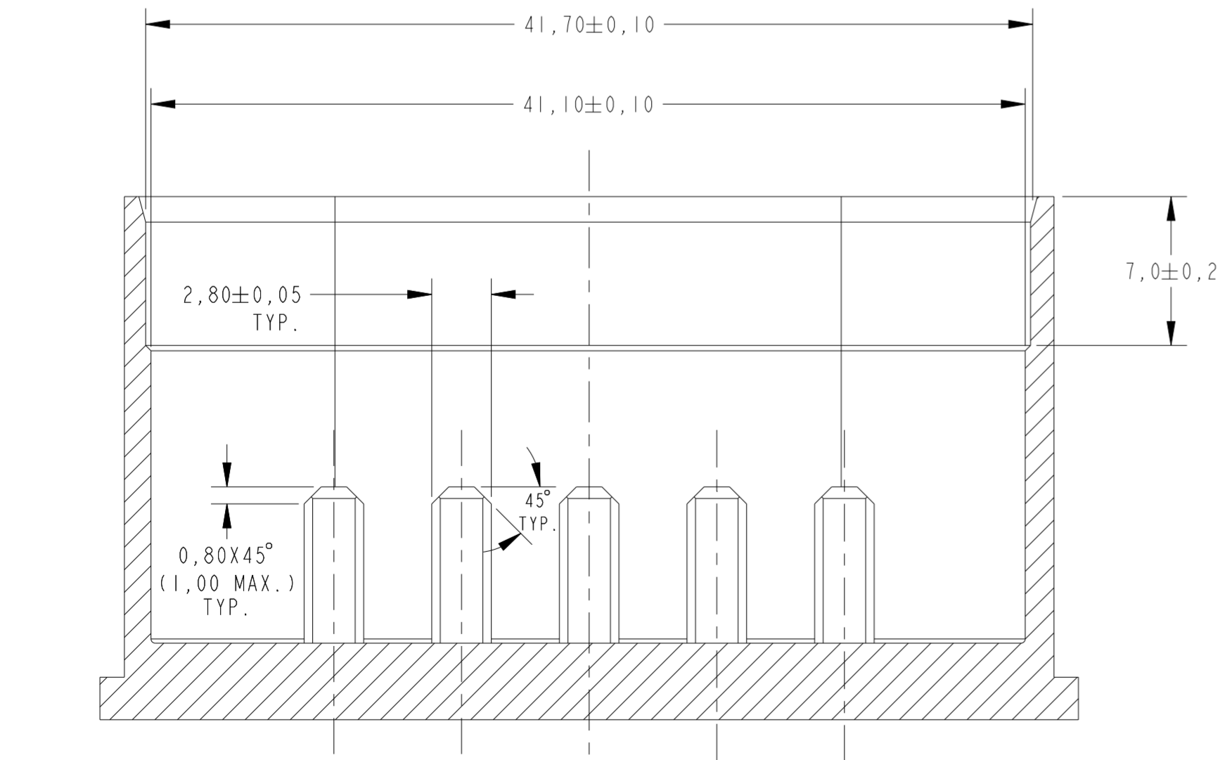
SECTION B-B
