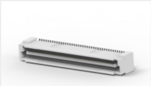
TE Part # CAT-313-PCB80 Free Height Plug Connector: Board-Board, Vertical, 80, 0.8mm
