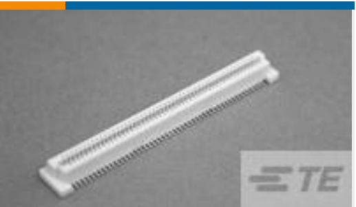
TE Part #640901-1 05P UMNL SOK HDR ASSY 94VO
