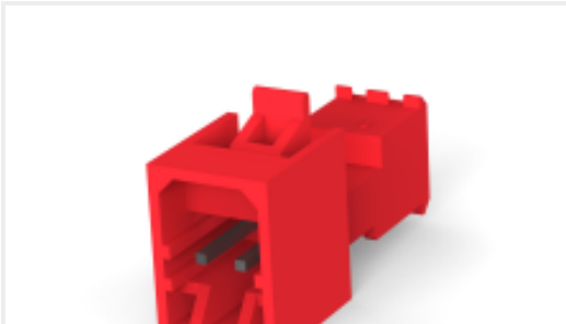
TE Part #CAT-104MTA-NTPMP MTA Plug: Nylon, Tin Plated, 2.54 mm, with Mating Alignment
