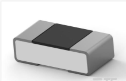
TE Part #6-2176364-8 RQ 0402 23K2 0.1% 10PPM 5K RL
