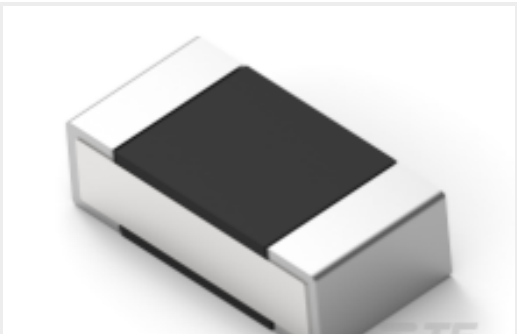
TE Part #1-2176305-1 RP 1E 0.1W 137R 0.1% 25PPM 5K RL
