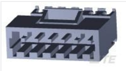
TE Part #3-641524-6 06P MTA156 POST CON ASSY LF
