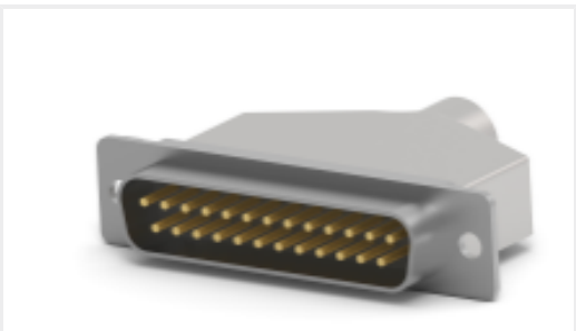
TE Part #CAT-AM7-248H4 IDC D-Sub: Connector Kit, Plug, Wire to Wire, Signal, 2.77 mm
