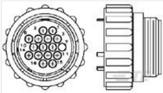
TE Part #206037-4 CPC PLUG ASSEMBLY SZ 17-16
