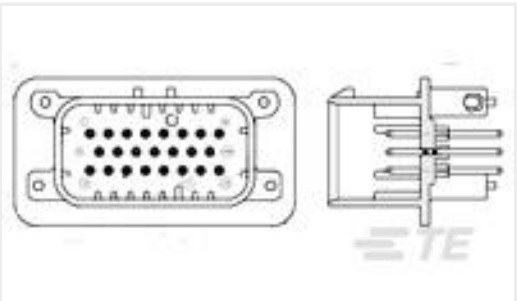
TE Part #1-776200-2 23POS,PIN DIA 1.3,HDR ASSY, 180DEG,COD 2
