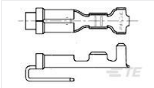
TE Part #62112-2 110 FASTON REC 22-18 AWG TPBR
