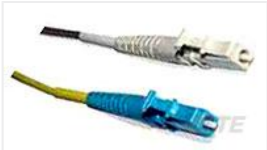
TE Part #6828129-1 CO KIT, LC, MM, DUP TIGHT
