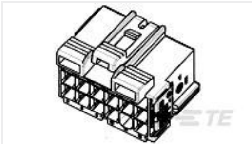
TE Part #1241581-1 JUN-POW-TIM HOUSING 17POS
