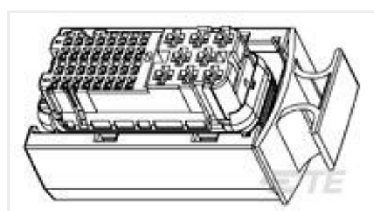
TE Part #368383-1 40P REC HSG ASSY() BLK
