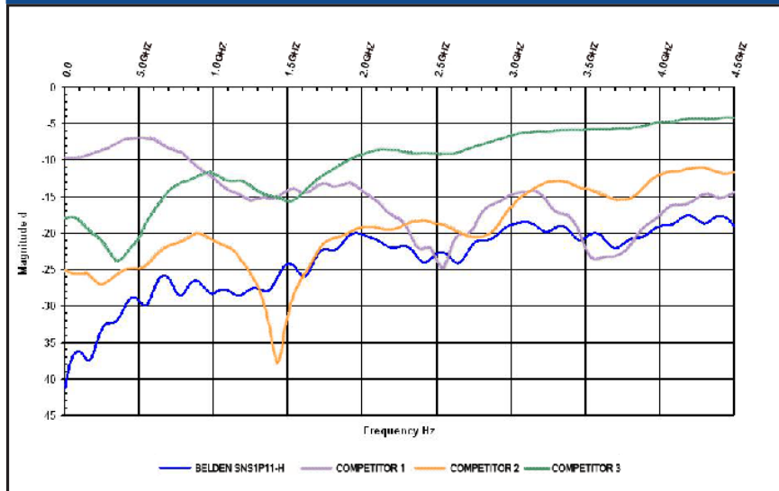
ProSNS™ RG-11 Connector RL Performance
