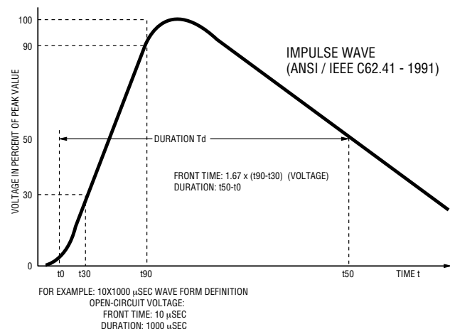
Figure 2. Surge Waveform
