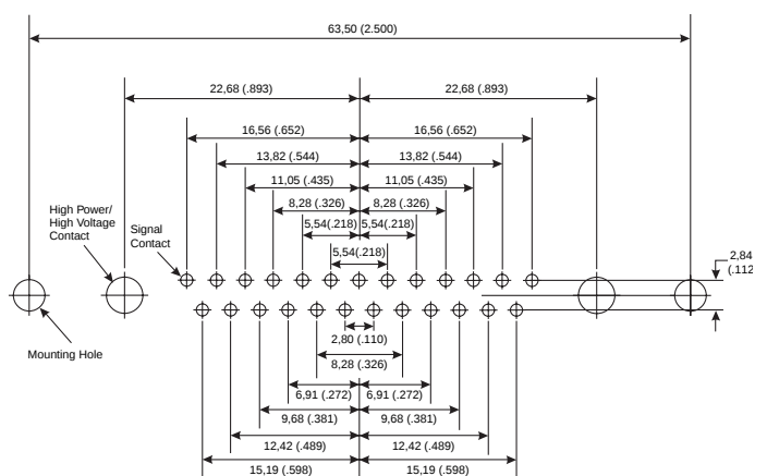
Signal Contact \varnothing Recommended PCB Hole \varnothing
