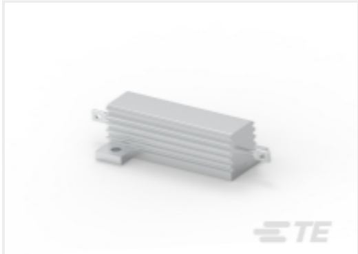
TE Part # 6-1630186-2 HSA50 18K 5%
