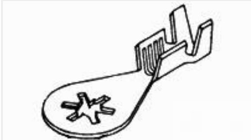
TE Part #62613-3 RING .190 12-10 AWG 024 TPCU
