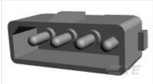
TE Part #350543-1 04P CMNL HDR ASSY SHORT NATL
