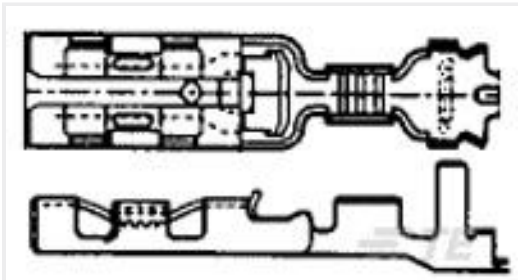
TE Part #353249-2 110 PL EX REC. 26-22AWG PTPHBZ
